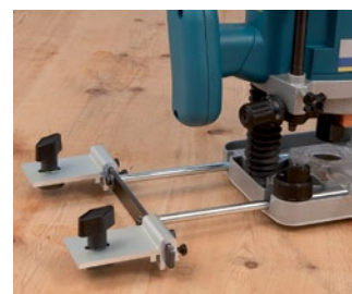
Adaptable to all Virutex routers by means of the optional adaptor 9045758.
