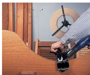
Possibility to band straight, circular or shaped pieces.
