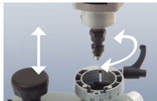
Simple adjustment of the height of the heads with the fine adjustment system.
