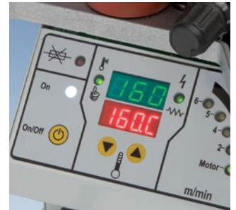
Temperature adjustment (120 to 200°C) controlled by microprocessor for higher accuracy on measurement.
